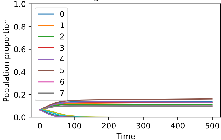
Evolution of strategies in Axelrod's 1st tournament
