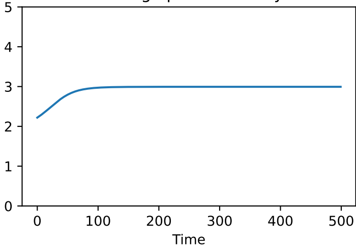
Average per turn utility
